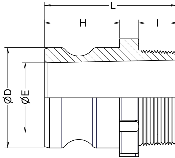
Section T-T
