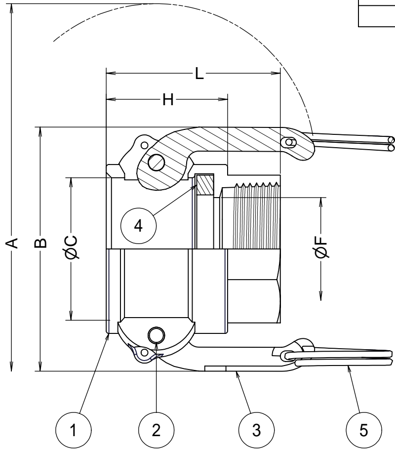
Section Q-Q
